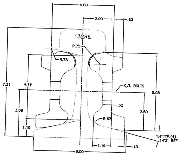
SECTION THROUGH JOINT BARS FULL SCALE-DIMENSIONS NOT GIVEN TO BE MFG.STANDARD
