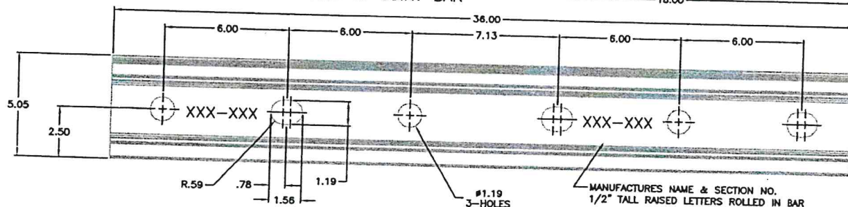
FRONT ELEVATION OF JOINT BAR QUARTER SCALE
