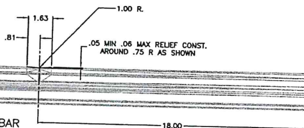
DETAIL OF HEAD 2 X SIZE
