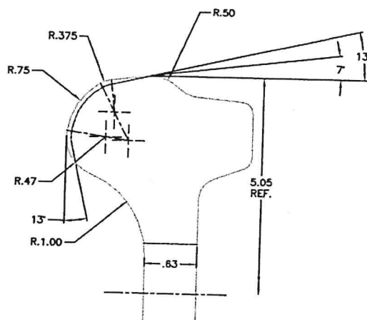
DETAIL OF HEAD 2 X SIZE
