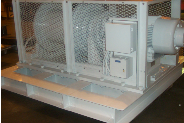
Winch Assembly
